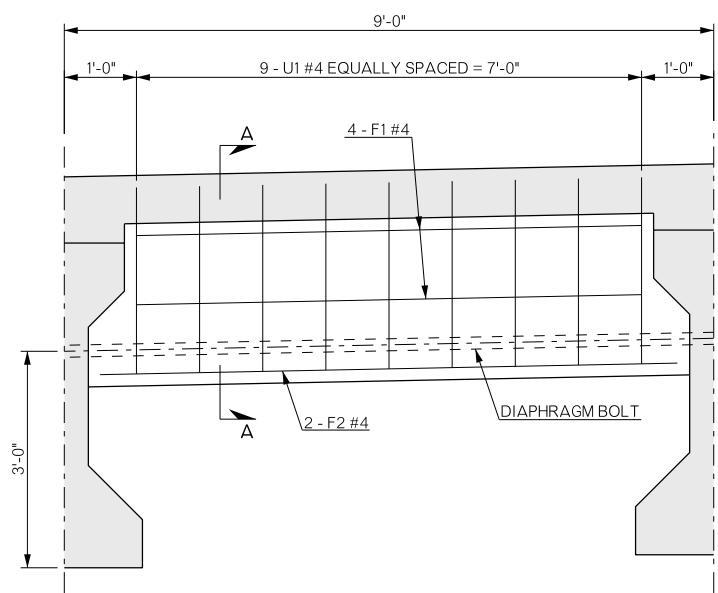
END DIAPHRAGM TYPE IV P.C. BEAM
