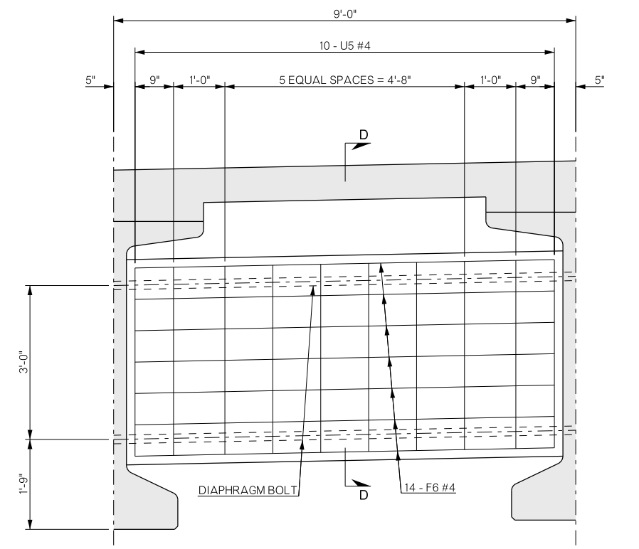
INTERMEDIATE DIAPHRAGM TYPE J P.C. BEAM
