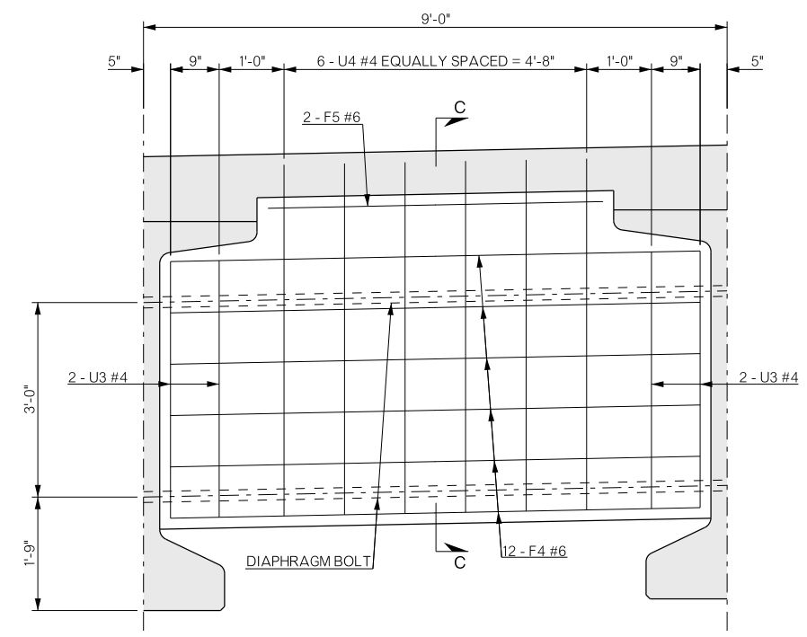
END DIAPHRAGM TYPE J P.C. BEAM
