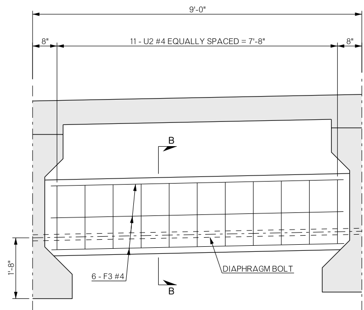
INTERMEDIATE DIAPHRAGM TYPE IV P.C. BEAM
